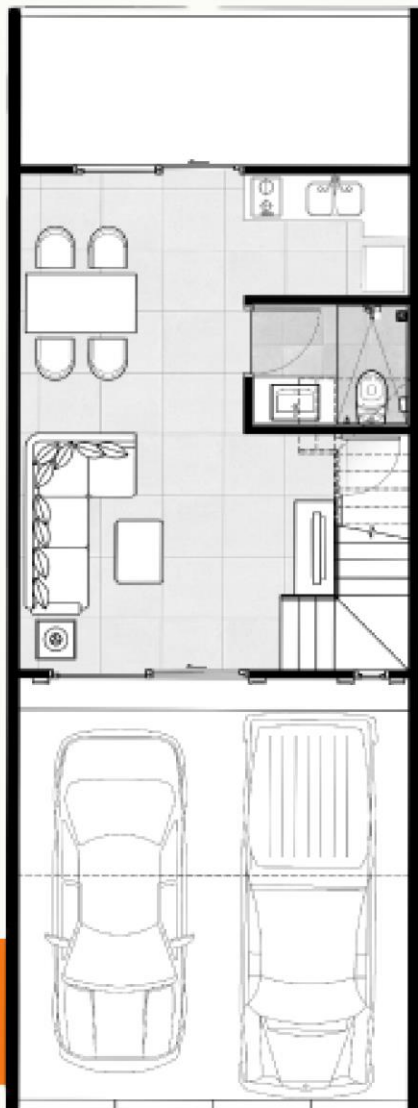
1 st Floor
