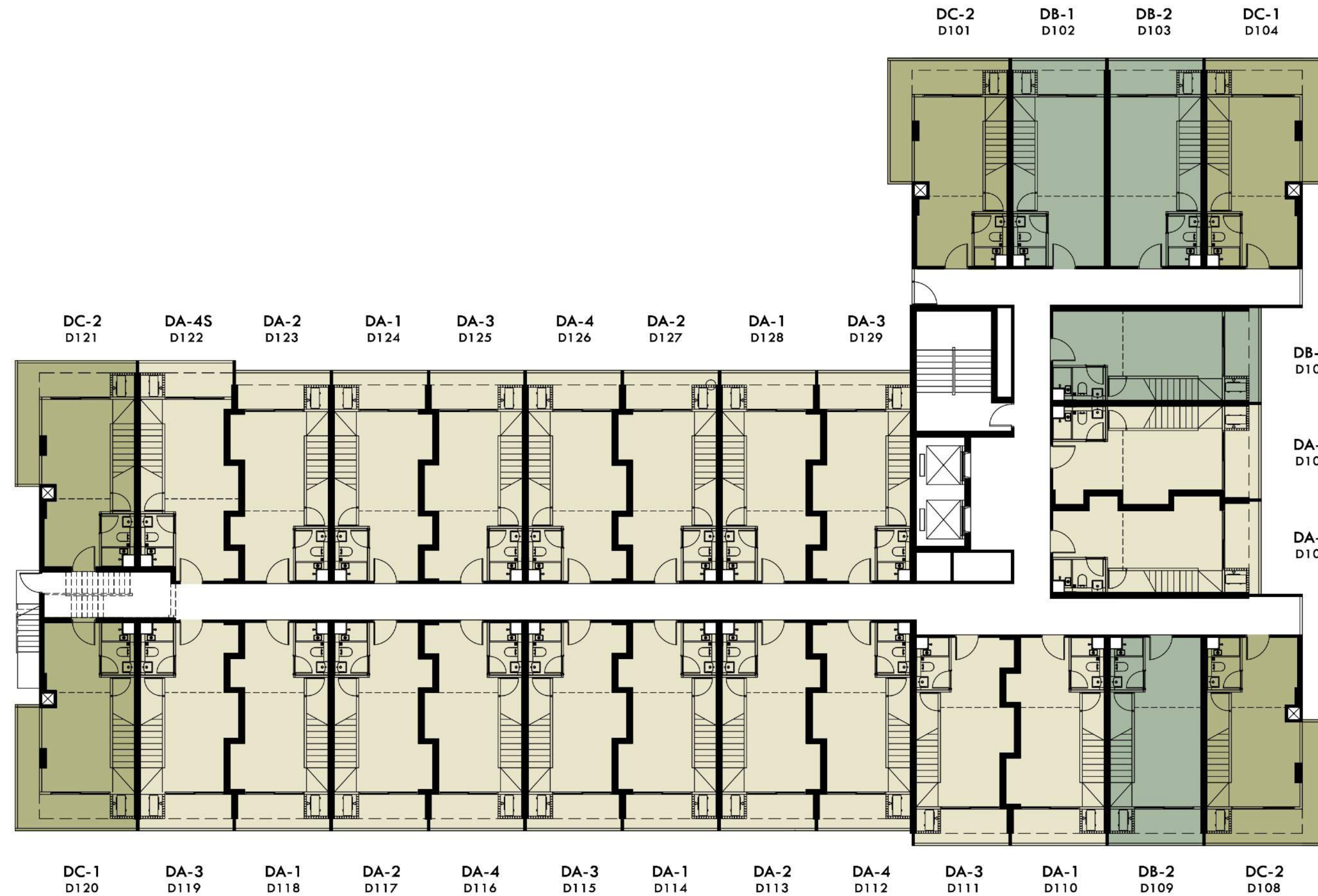
BUILDING D GROUND FLOOR PLAN
