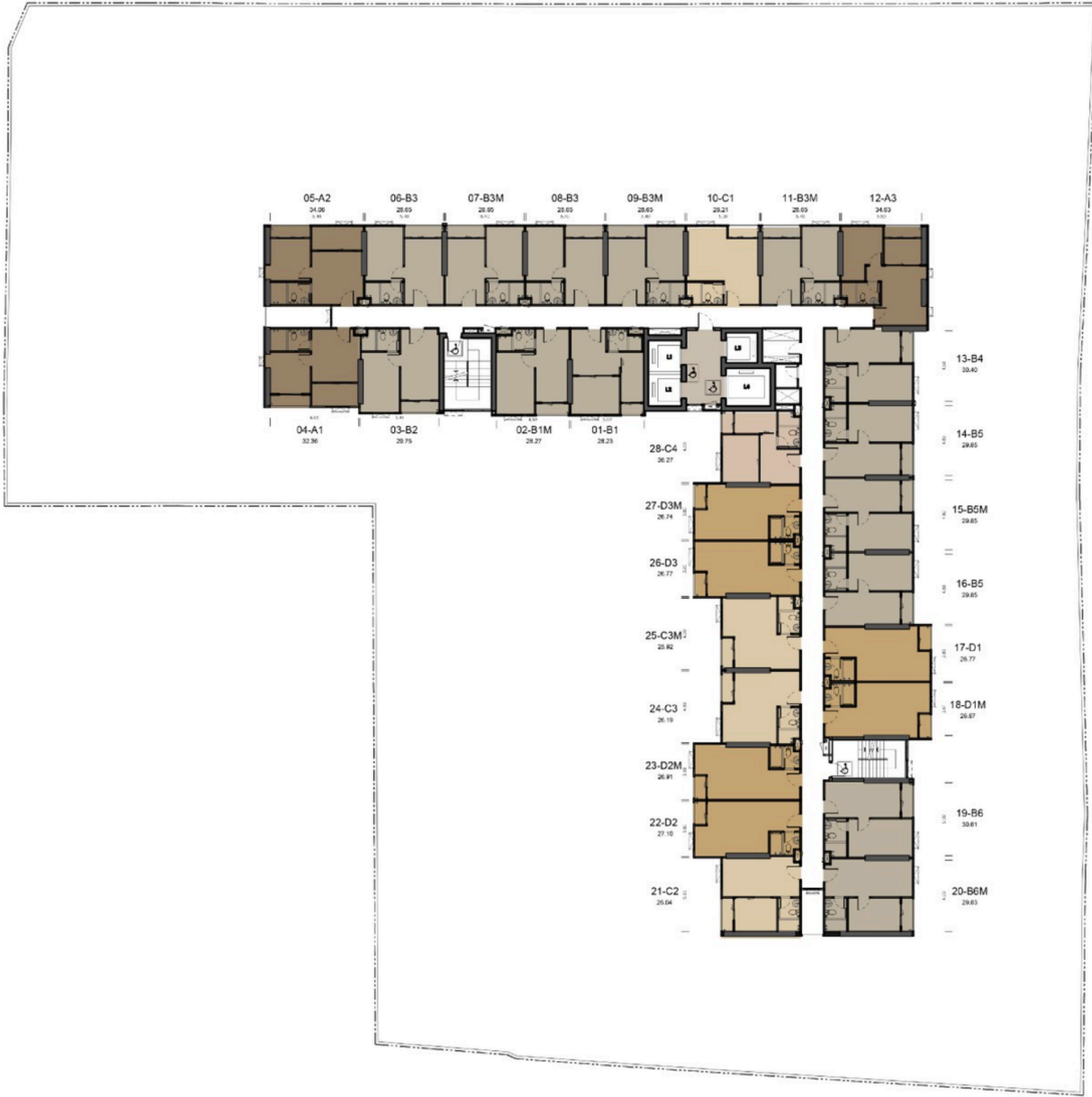
8TH.-12TH. FLOOR SCALE 1:400
